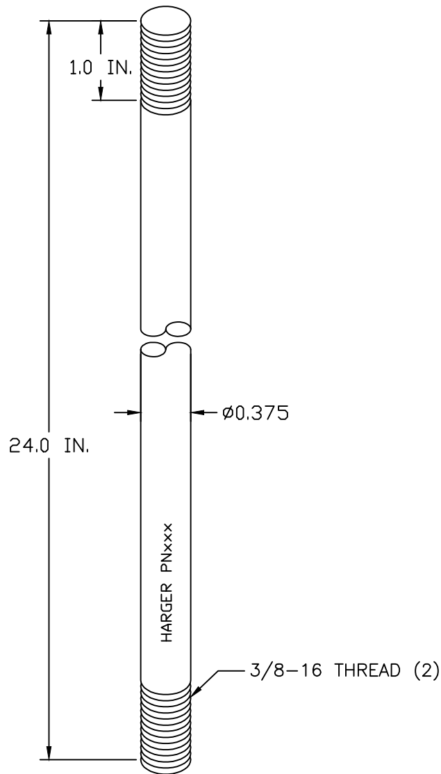
COPPER AIR TERMINAL EXTENSION
