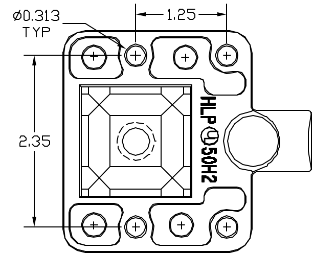
BASE DETAIL
