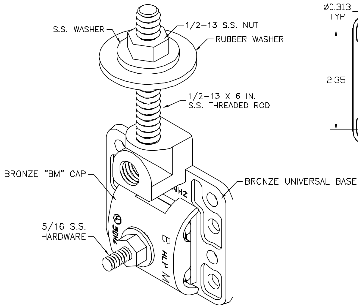
CONCEALED BASE ASSEMBLY
