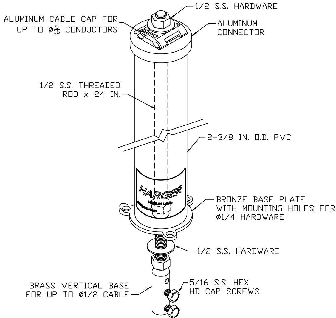
BI-METAL VERTICAL THRU ROOF ALUMINUM ROOF CONDUCTOR TO COPPER DOWNLEAD
