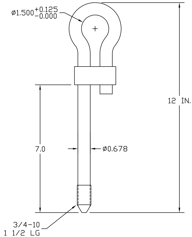
COPPER CLAD TIE DOWN GROUND ROD
