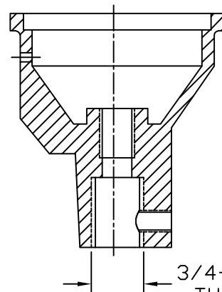
SECTION A-A BRONZE FLOOR GROUND RECEPTACLE
