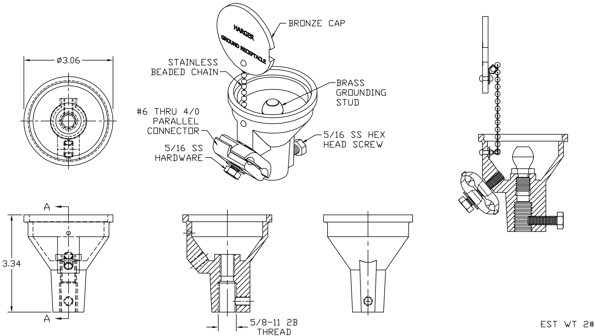
SECTION A-A BRONZE FLOOR GROUND RECEPTACLE
