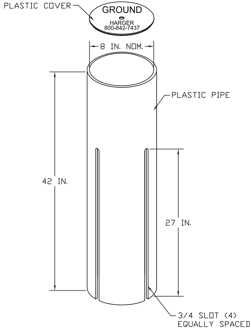
PVC SLOTTED WELL W/PLASTIC COVER
