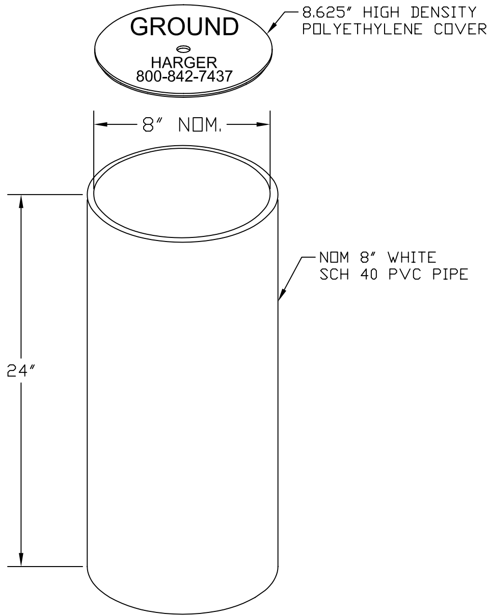
PVC WELL W/ HDPE COVER
