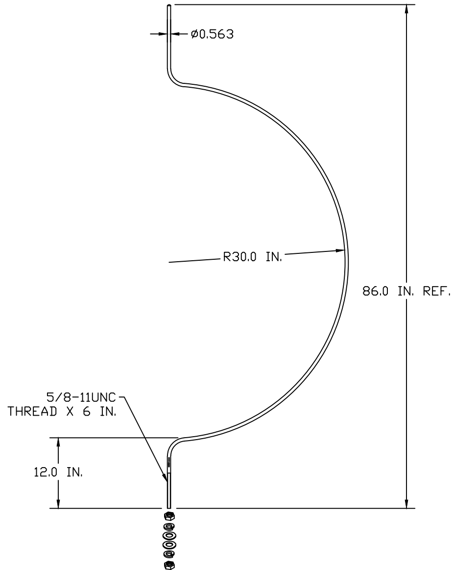
BENT COPPER CLAD AIR TERMINAL
