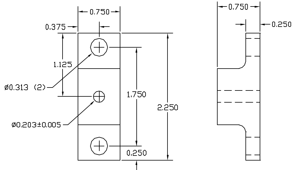
DELRIN WHITE INSULATOR
