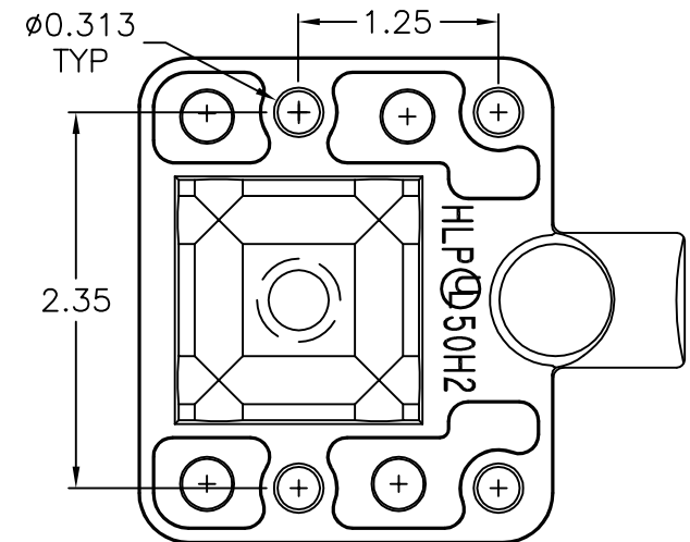
BASE DETAIL
