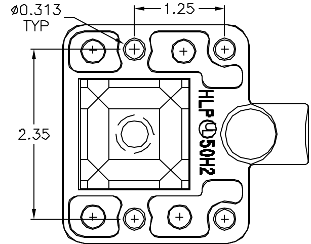
BASE DETAIL
