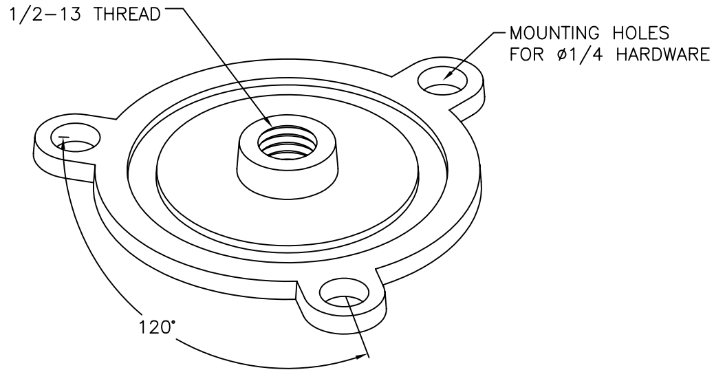
ALUMINUM VERTICAL THRU-ROOF BASE PLATE FOR 2" SCHEDULE 40 PVC PIPE
