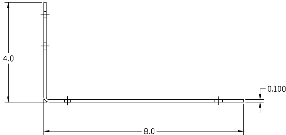
ALUMINUM CABLE CLIP FOR A24 AND A28 LIGHTNING CONDUCTOR
