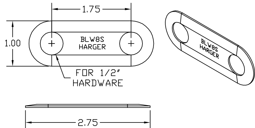
STAINLESS STEEL CUPPED WASHER
