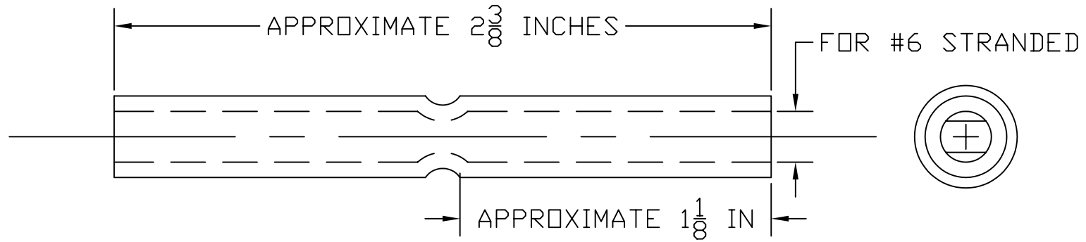
6 AWG SOLID (ø0.184) LONG BARREL BUTT SPLICE
