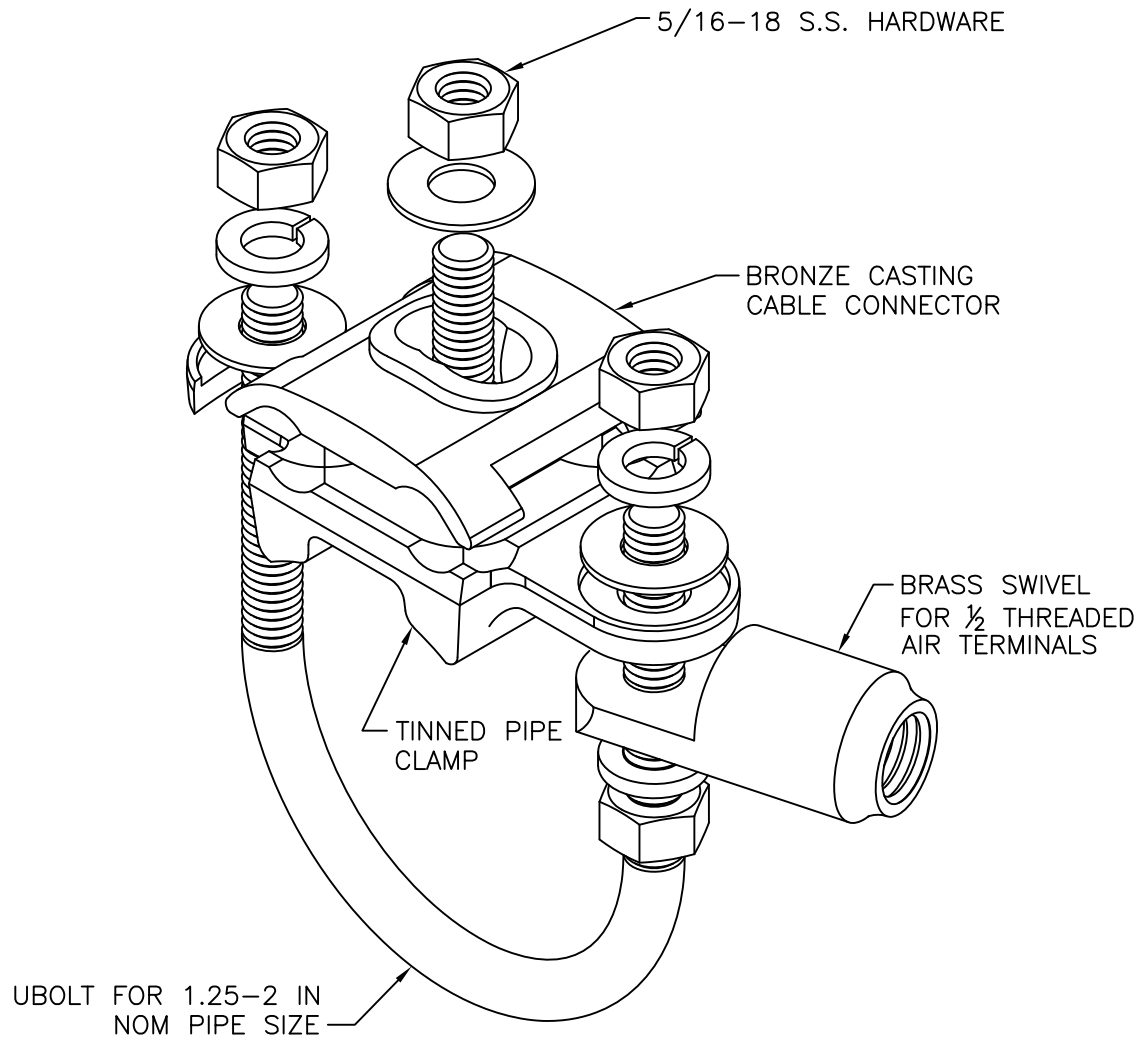
1 1/2- 2" PIPE CLAMP FOR 1/2" AIR TERMINAL
