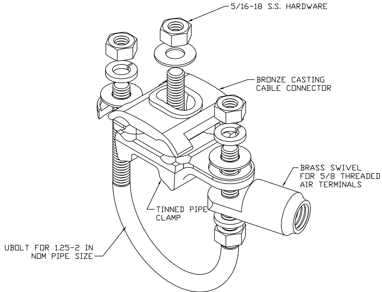
1 1/2- 2" PIPE CLAMP FOR 5/8" AIR TERMINAL
