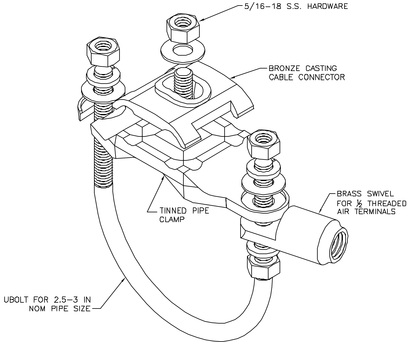
2 1/2-3" PIPE CLAMP FOR 1/2" AIR TERMINAL
