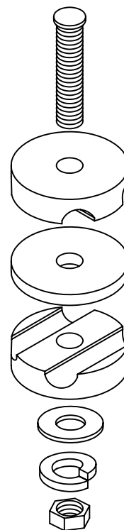
ASSEMBLY SCALE 1:2
