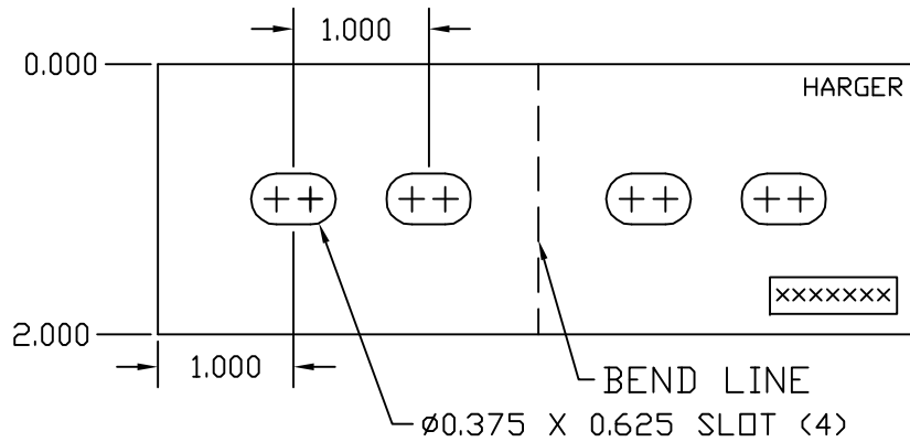
FLAT LAYOUT
