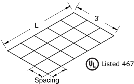
UL Listed Prefabricated #8 Solid Copper Ground Mesh
