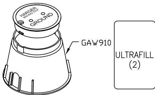
GROUND ACCESS WELL & ULTRAWELD
