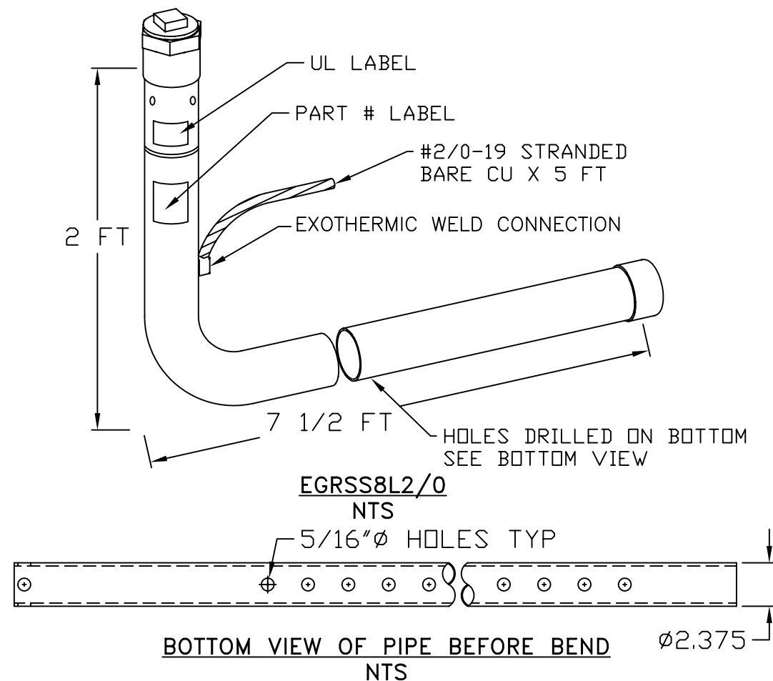
S.S. L SHAPED ENHANCED GROUND ROD
