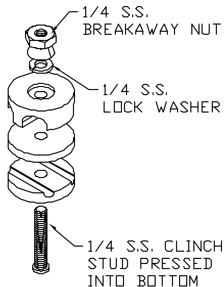
ASSEMBLY
