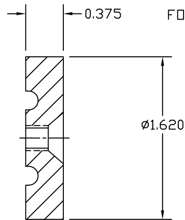
BOTTOM, BRASS TIN PLATED
