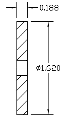
SPACER, BRASS TIN PLATED
