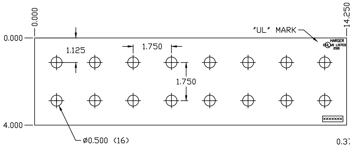
COPPER GROUND BAR
