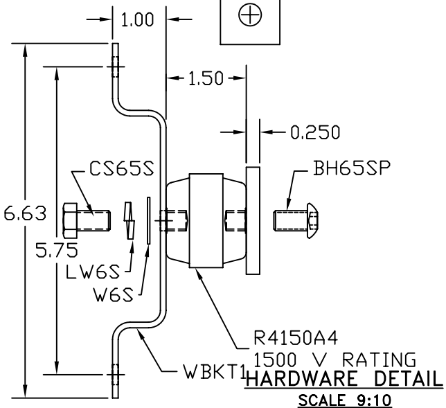
HARDWARE DETAIL SCALE 9:10
