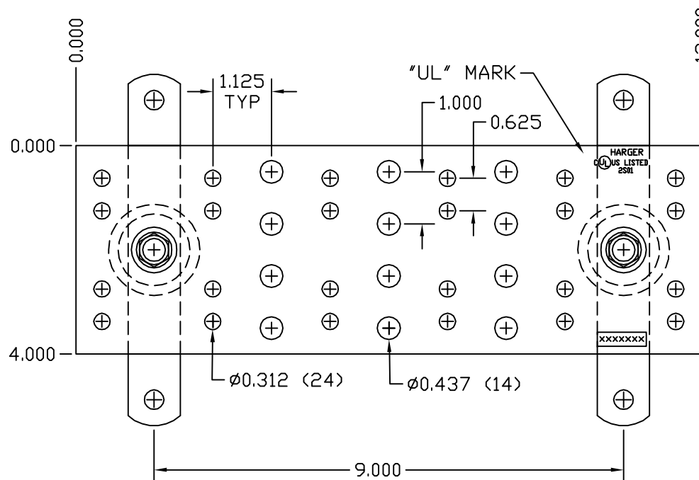
COPPER GROUND BAR ASSEMBLY
