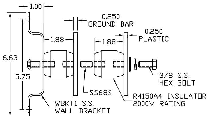
COPPER GROUND BAR ASSEMBLY
