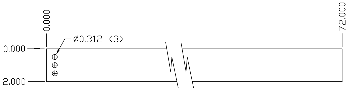
2" X .016" FLAT STRAP (1)
