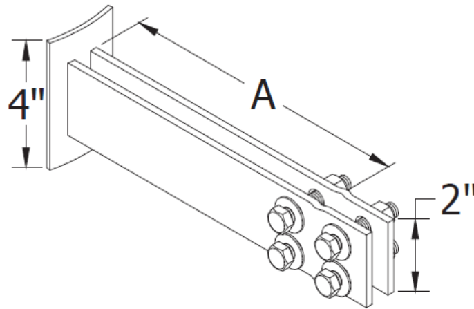
LRCSS3/16X8 Lightning Rod Clamp
