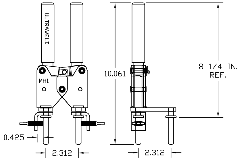
ASSEMBLY DETAIL
