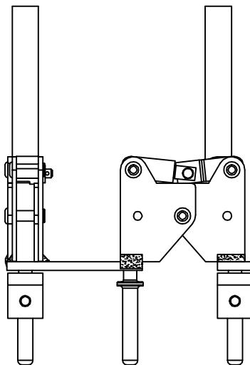
RIVETING DETAIL
