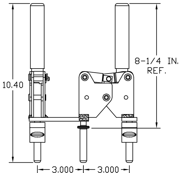
ASSEMBLY DETAIL
