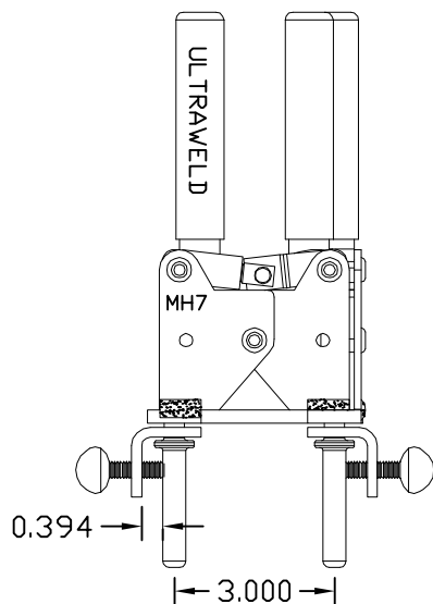
ASSEMBLY DETAIL
