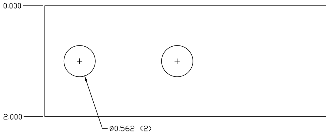
FLAT LAYOUT
