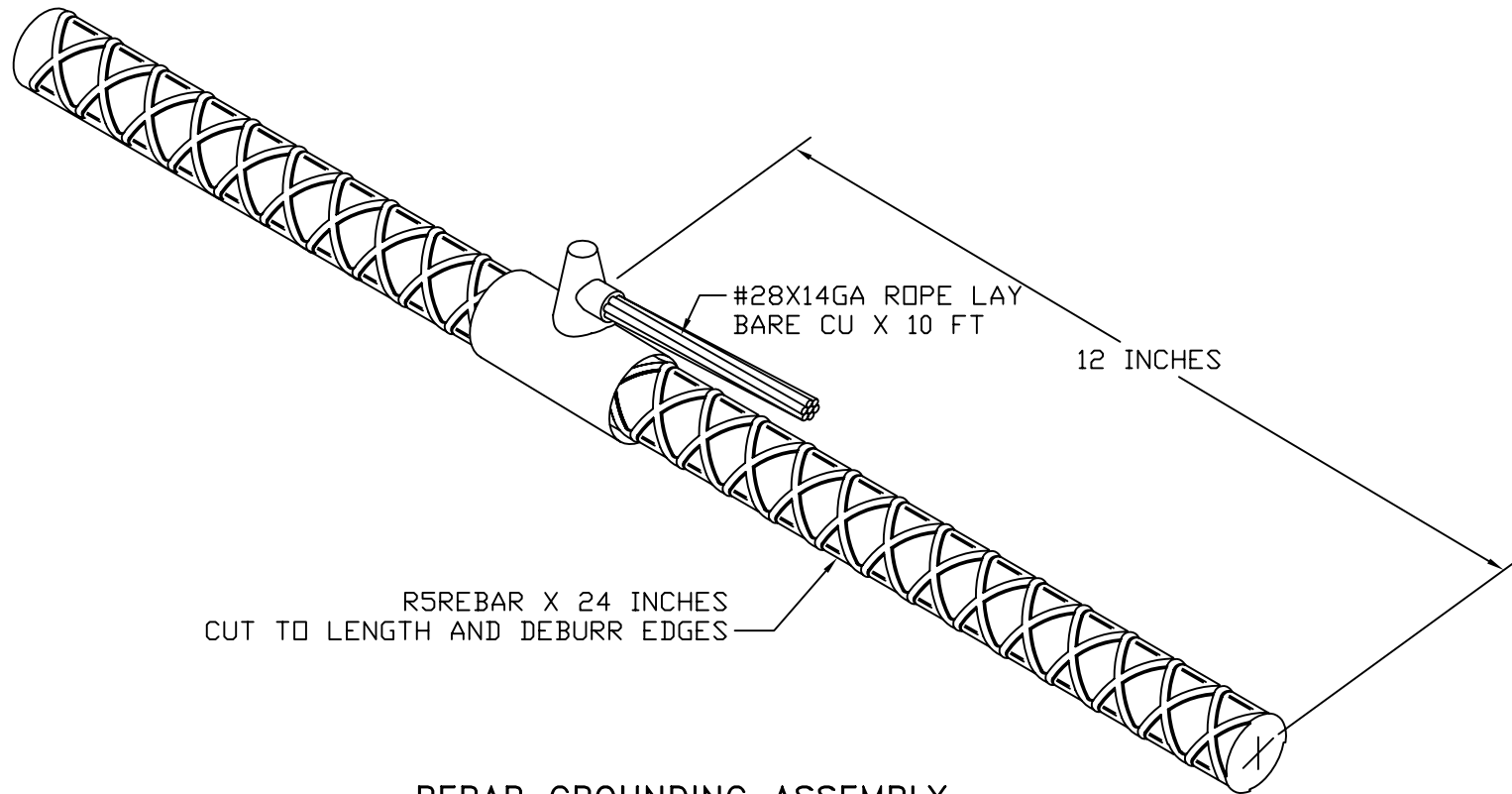
REBAR GROUNDING ASSEMBLY
