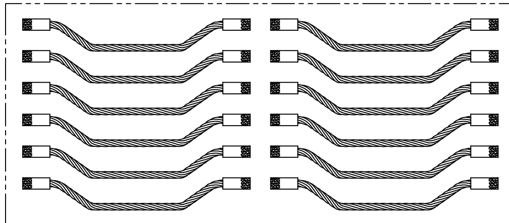
3/16x7.5 TAB STYLE RAIL BONDS (100) PCS
