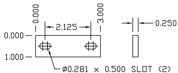
COPPER SPLICE PLATE
