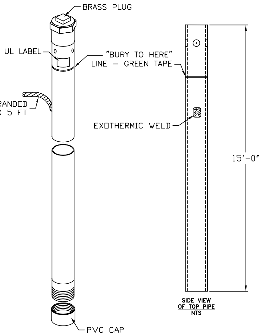
TOP PIECE OF SEGR304/0 NTS
