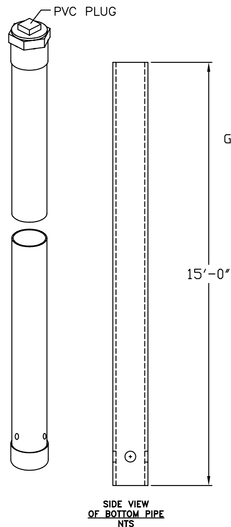
BOTTOM PIECE OF SEGR304/0 NTS
