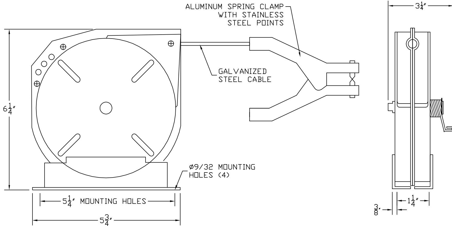
RETRACTABLE REEL WITH 20 FT OF CABLE
