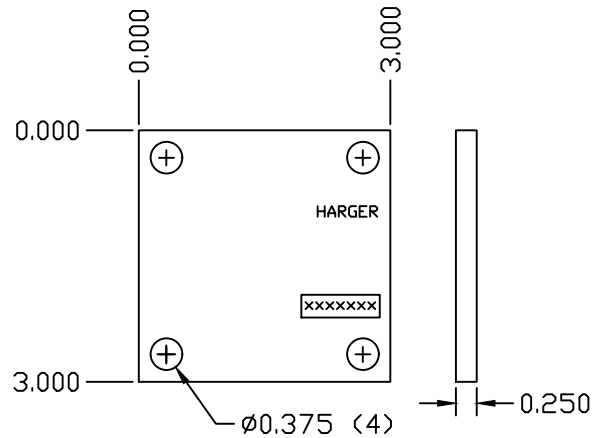
NUT PLATE (2)
