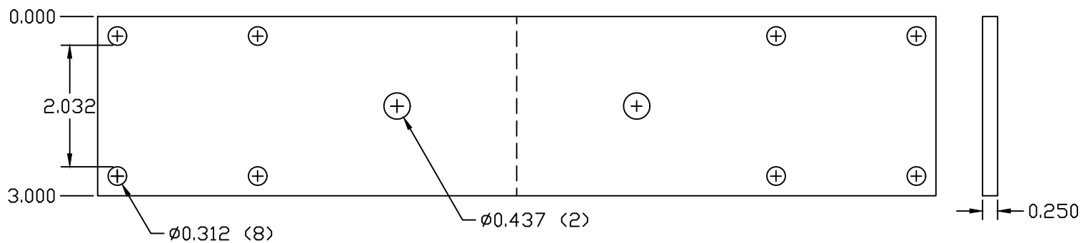
FLAT BAR LAYOUT (1)
