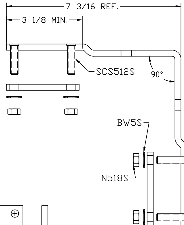
ASSEMBLY
