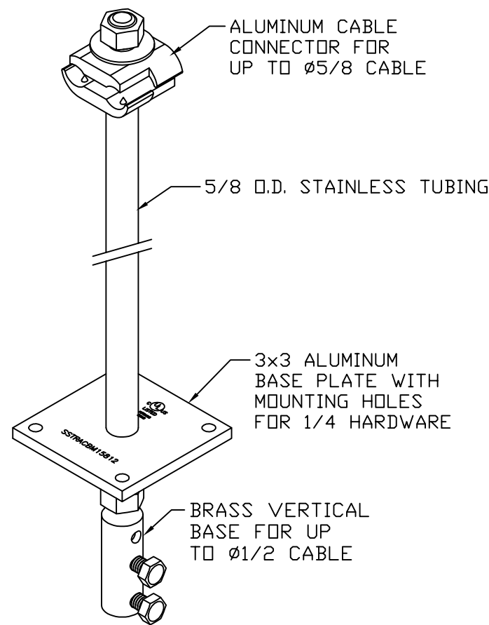
ASSEMBLY VIEW FOR REFERENCE SHIPS PARTIALLY ASSEMBLED
