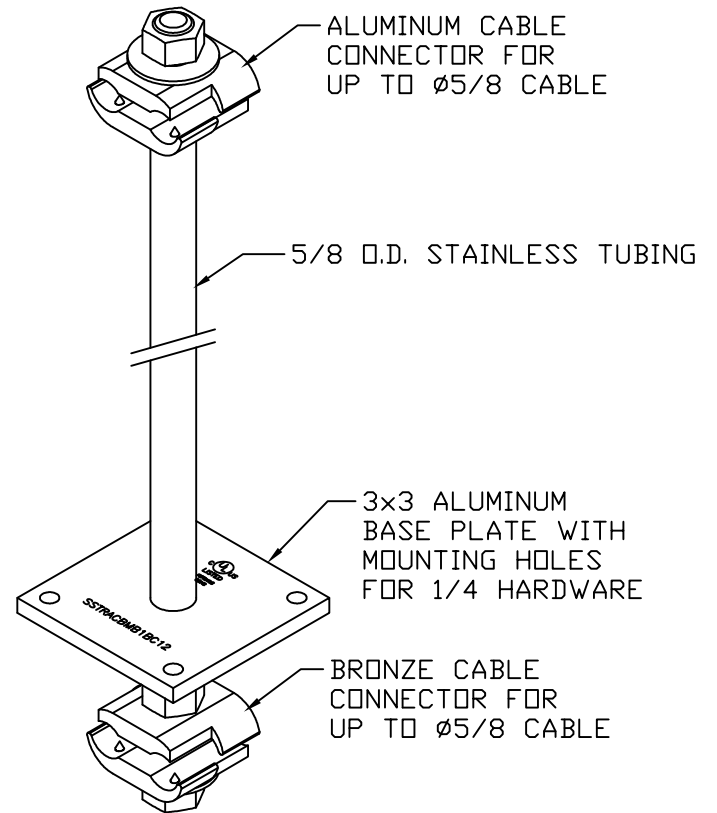
ASSEMBLY VIEW FOR REFERENCE SHIPS PARTIALLY ASSEMBLED
