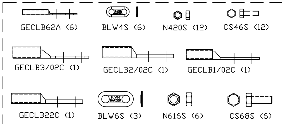
HARDWARE KIT
