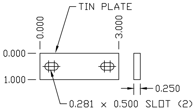
COPPER SPLICE PLATE
