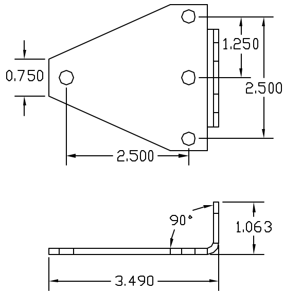
BRACKET DETAIL
