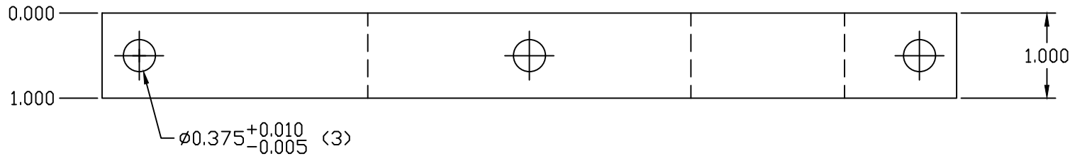
FLAT LAYOUT
