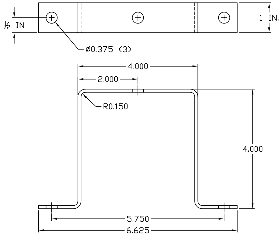
WALL BRACKET
